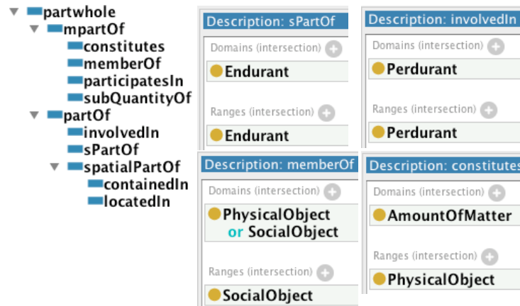
Fig. 2. The OWLized version of the taxonomy of part-whole relations [15] (left) with screenshots of domain and range restrictions of four object properties (right).
